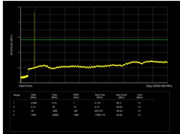
LTE Band 25 1.4MHz CH-Middle 9kHz~20GHz
