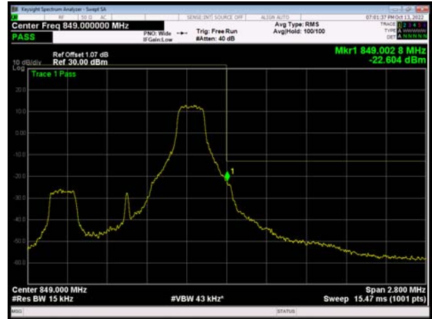
LTE Band 26 16QAM 1.4MHz CH-High 100%RB
