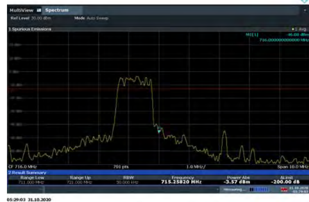
LTE Band 85 QPSK 5MHz CH-High, 100%RB
