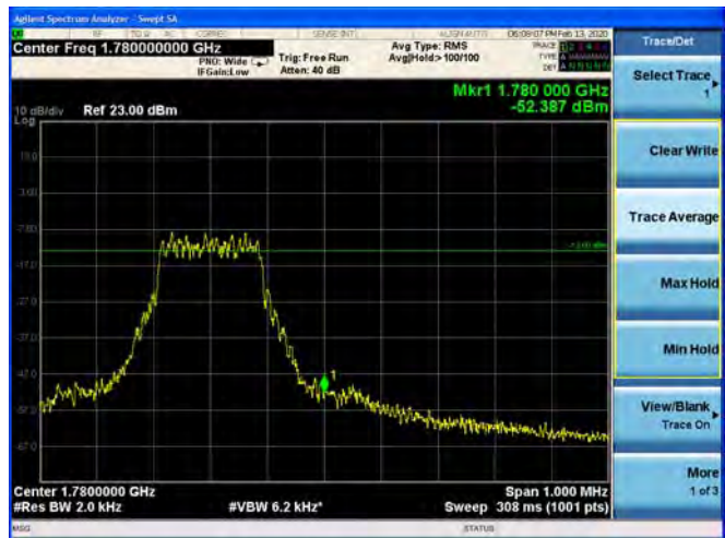
NB-IOT Band 66 QPSK 15KHz 12@0 CH-High
