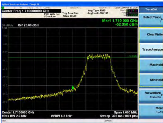
NB-IOT Band 66 QPSK 15KHz 12@0 CH-Low
