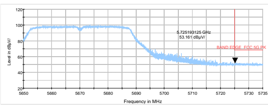
802.11n HT40-Channel 134: Peak
