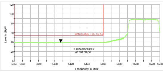
802.11n HT40-Channel 102: Average
