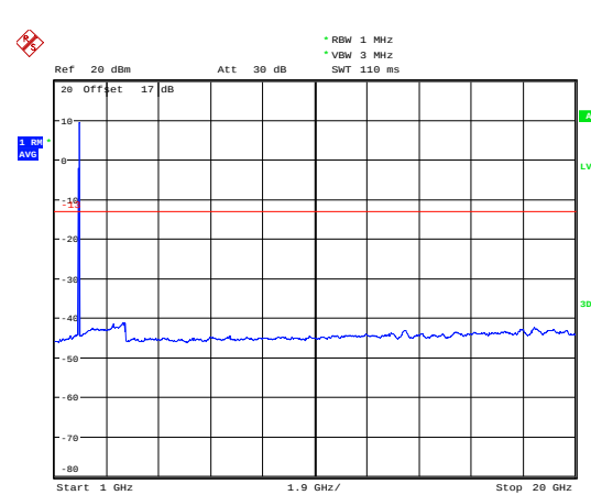
LTE Band 25 1.4MHz CH-Middle 1GHz~20GHz
