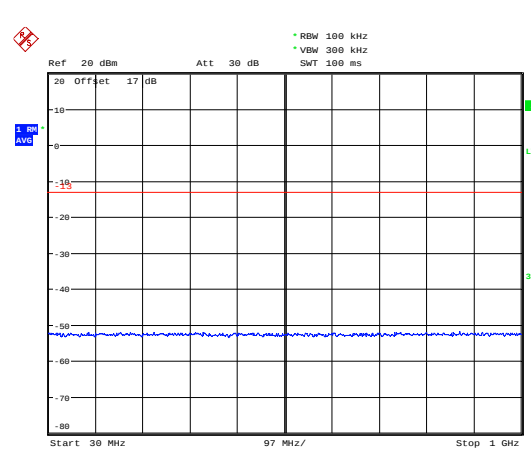
LTE Band 25 1.4MHz CH-Middle 30MHz~1GHz
