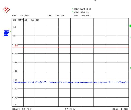
LTE Band 251.4MHz CH-High 30MHz~1GHz
