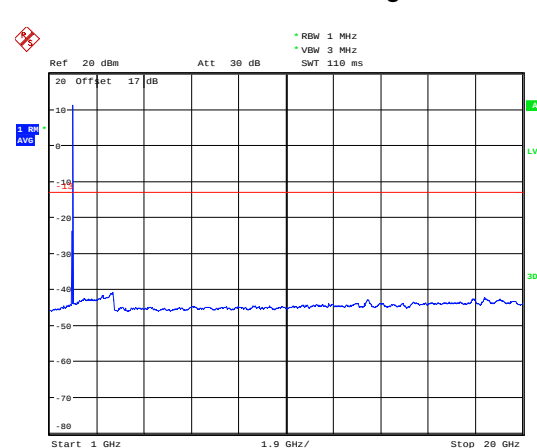
LTE Band 25 1.4MHz CH-High 1GHz~20GHz
