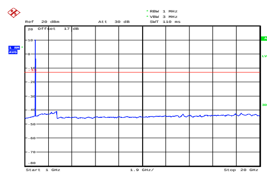
LTE Band 25 1.4MHz CH-Low 1GHz~20GHz
