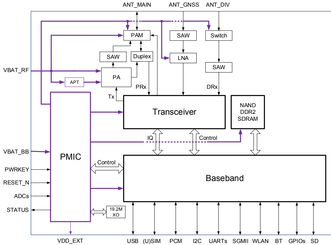
Figure 1: Functional Diagram
