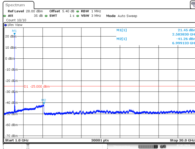
Band41_20MHz_16QAM_40620_1RB#0
