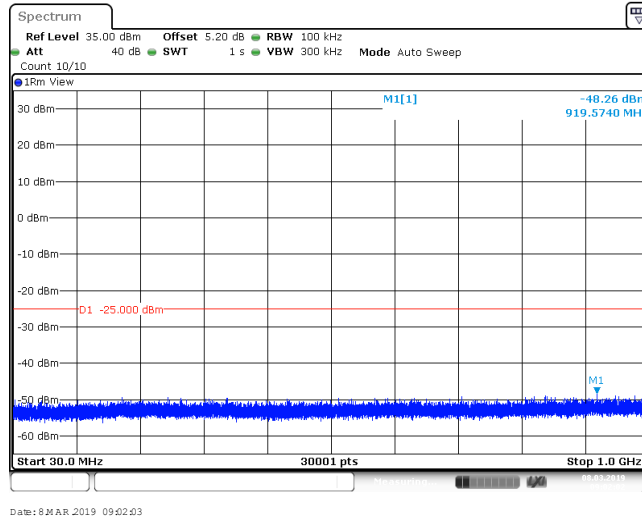
Band41_20MHz_64QAM_40620_1RB#0
