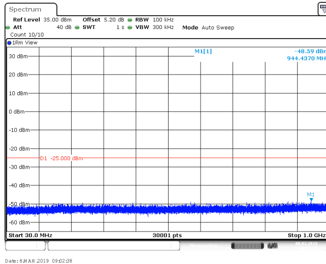
Band41_20MHz_64QAM_41490_1RB#0
