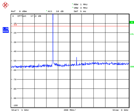
LTE Band 66 1.4MHz CH--Low 1GHz ~3GHz
