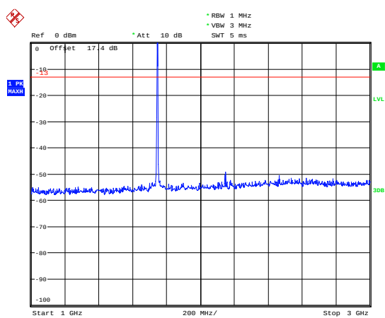
LTE Band 66 1.4MHz CH-Middle 1GHz ~3GHz
