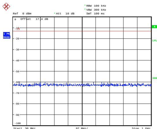
LTE Band 66 1.4MHz CH-Low 30MHz~1GHz
