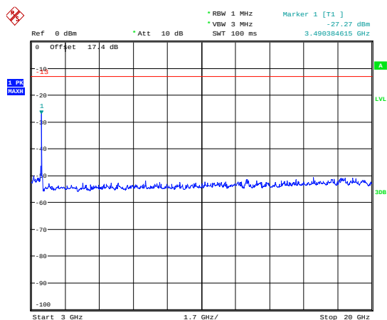
LTE Band 66 1.4MHz CH- Middle 3GHz ~20GHz
