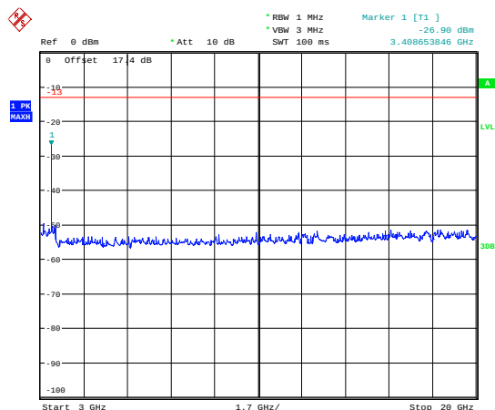
LTE Band 66 1.4MHz CH--Low 3GHz ~20GHz
