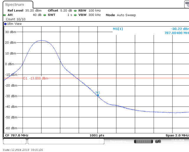
Band13_10MHz_QPSK_23230_Right_50RB#0
