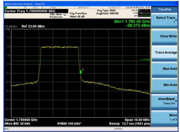
LTE Band 66 16QAM 5MHz CH-High, 1 RB
