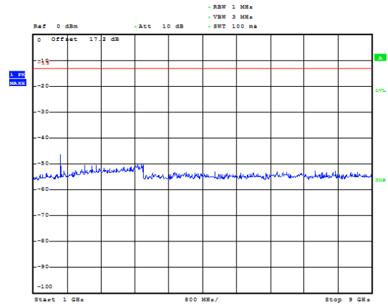
LTE Band 5 10MHz CH-Low 1GHz~9GHz
