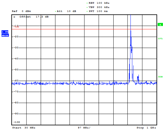
LTE Band 5 10MHz CH-Low 30MHz~1GHz
