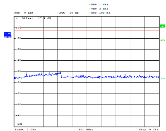
LTE Band 5 10MHz CH-High 1GHz~9GHz
