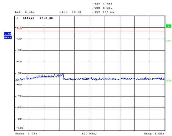
LTE Band 5 10MHz CH-Middle 1GHz~9GHz
