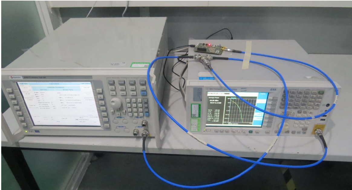
Conducted Testing Setup
