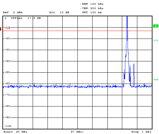
WCDMA Band V CH-Middle 30MHz ~ 1GHz
