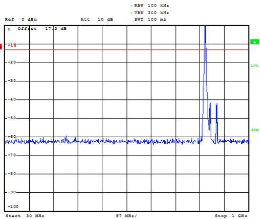
WCDMA Band V CH-Low 30MHz ~ 1GHz
