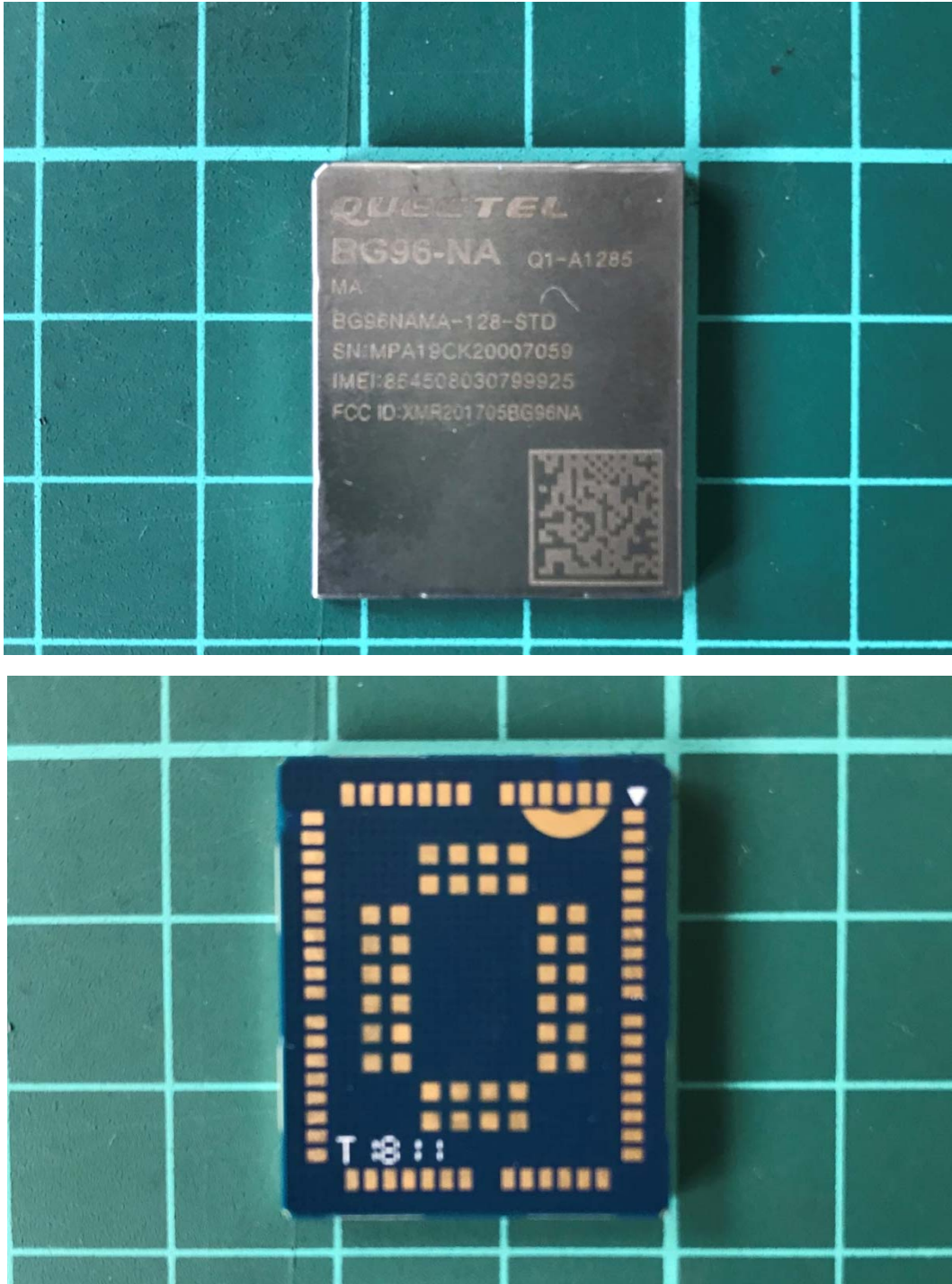
Picture 1 EUT
