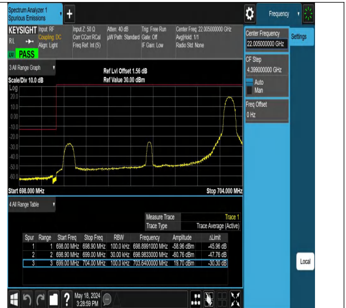
Band12_5MHz_QPSK_23035_1RB#24
