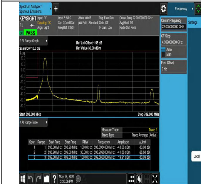
Band12_10MHz_QPSK_23060_1RB#0
