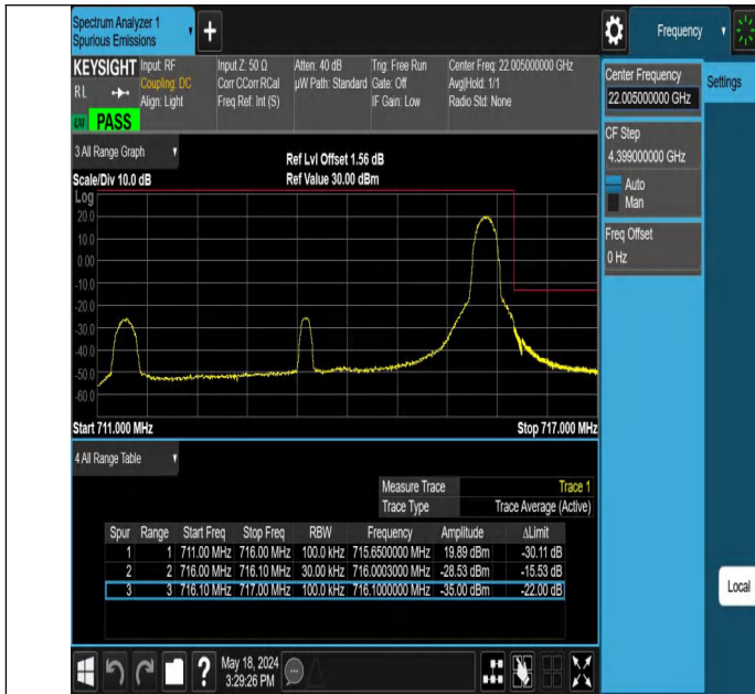
Band12_5MHz_QPSK_23155_1RB#24
