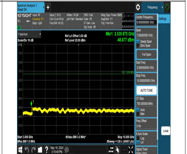
Band12_1.4MHz_QPSK_23095_1RB#5_3000~10000_3000~1000
