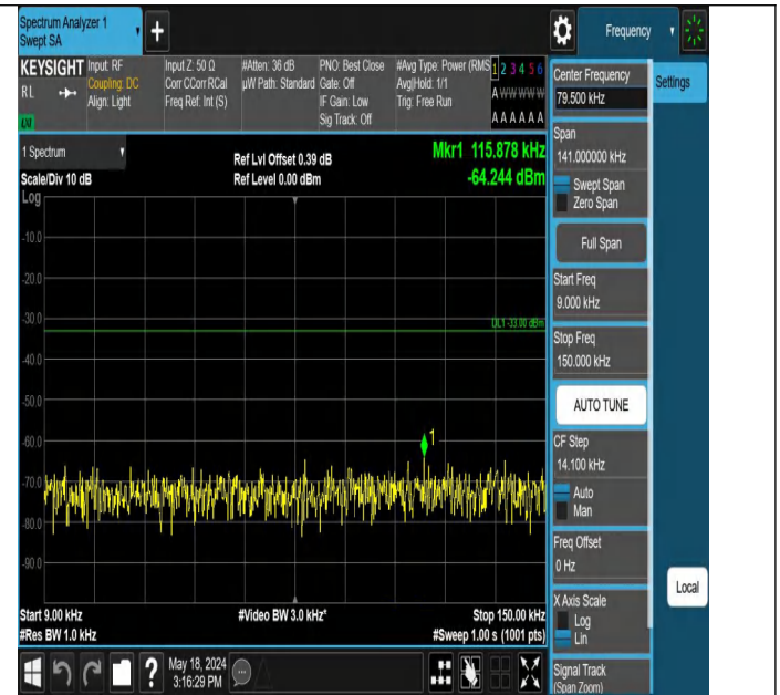
Band12_1.4MHz_QPSK_23173_1RB#5_0.009~0.15_0.009~0.15
