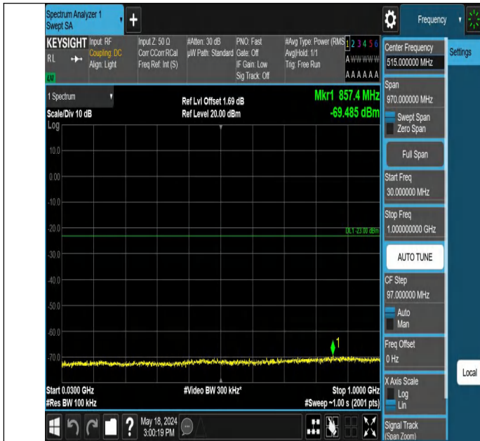
Band4_15MHz_QPSK_20175_1RB#0_30~1000_30~1000
