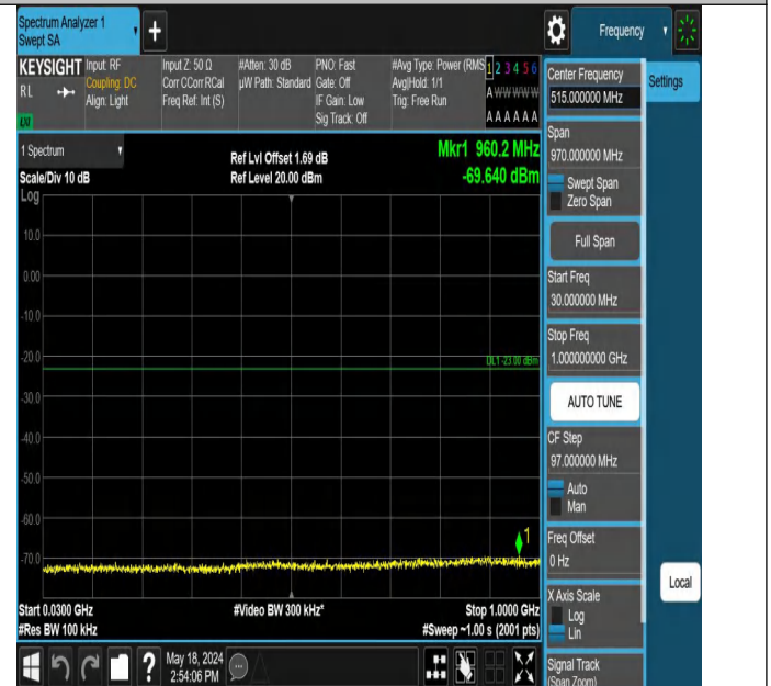
Band4_10MHz_QPSK_20175_1RB#49_30~1000_30~1000
