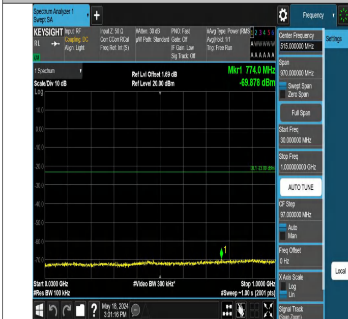
Band4_15MHz_QPSK_20325_1RB#0_30~1000_30~1000
