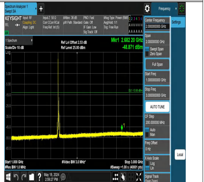
Band4_15MHz_QPSK_2025_1RB#0_1000~3000_1000~3000
