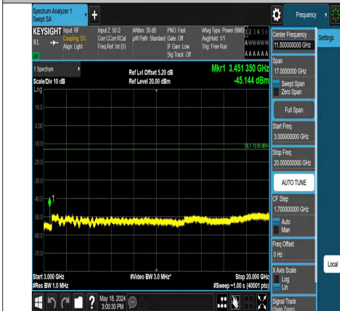
Band4_15MHz_QPSK_20175_1RB#0_3000~20000_3000~20000
