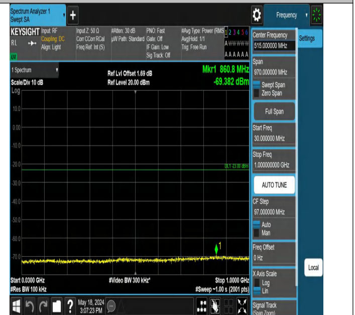
Band4_20MHz_QPSK_20175_1RB#99_30~1000_30~1000
