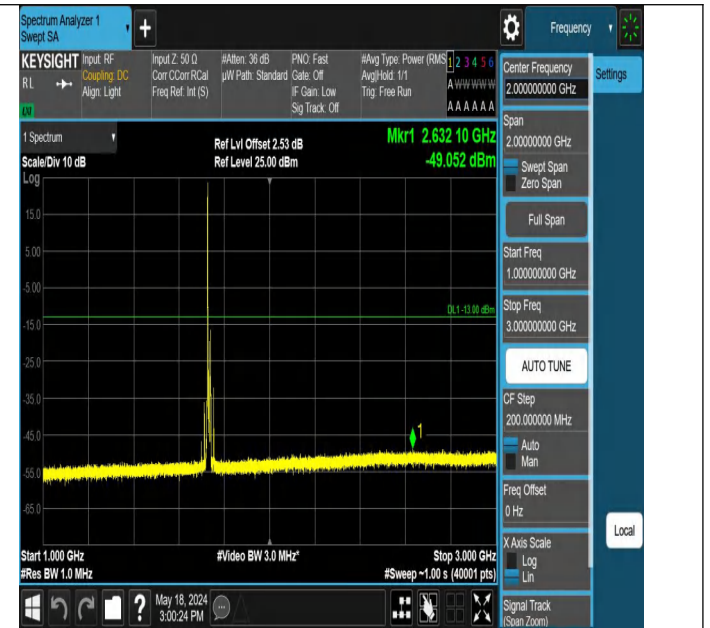
Band4_15MHz_QPSK_20175_1RB#0_1000~3000_1000~3000
