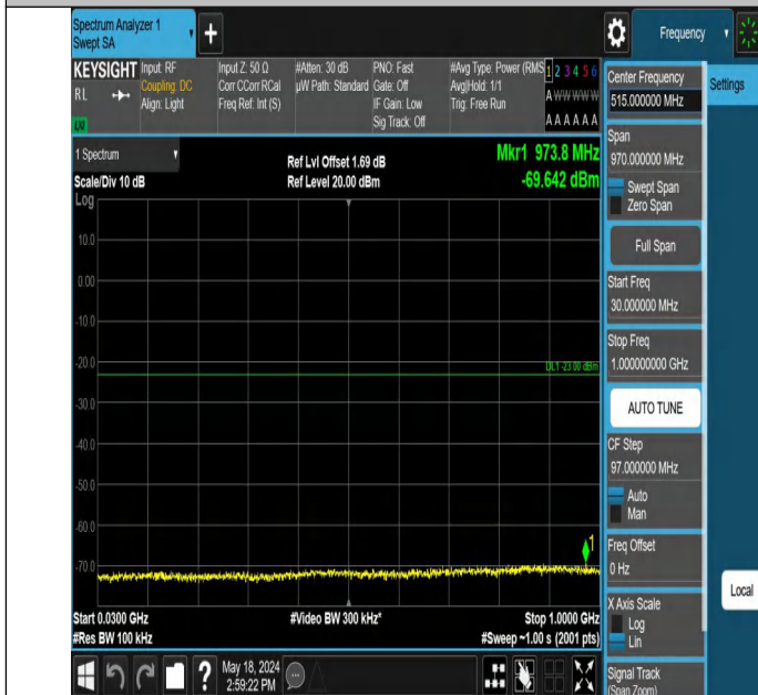
Band4_15MHz_QPSK_2025_1RB#0_30~1000_30~1000
