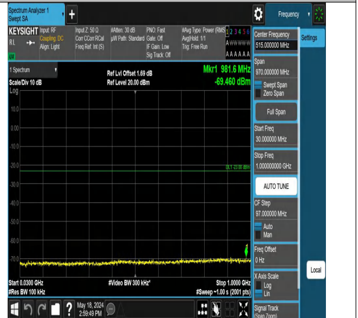
Band4_15MHz_QPSK_20025_1RB#74_30~1000_30~1000
