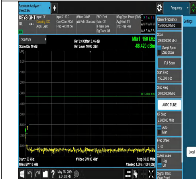
Band4_10MHz_QPSK_20175_1RB#49_0.15~30_0.15~30
