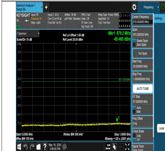
Band4_20MHz_QPSK_20175_1RB#0_30~1000_30~1000
