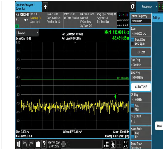
Band4_15MHz_QPSK_2025_1RB#0_0.009~0.15_0.009~0.15
