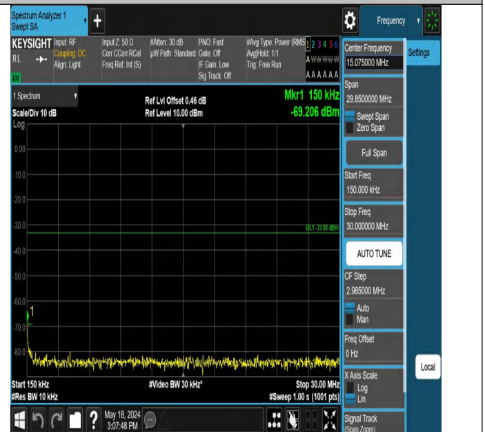
Band4_20MHz_QPSK_20300_1RB#0_0.15~30_0.15~30
