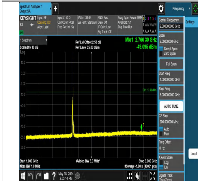
Band4_10MHz_QPSK_20000_1RB#49_1000~3000_1000~3000
