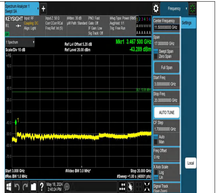
Band4_3MHz_QPSK_20175_1RB#14_3000~20000_3000~20000
