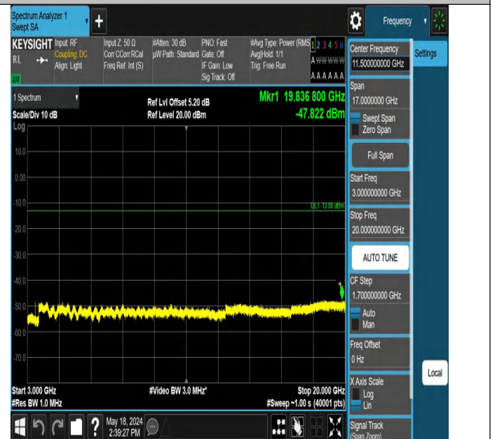
Band4_3MHz_QPSK_19965_1RB#14_3000~20000_3000~20000
