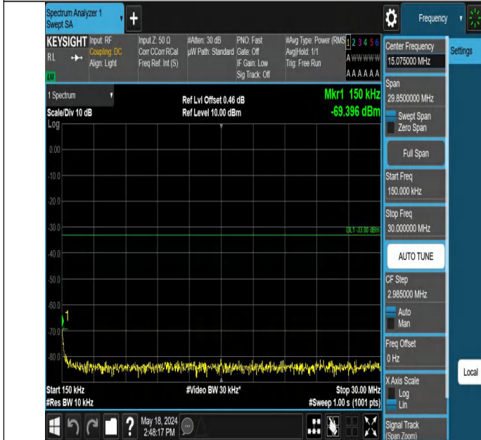
Band4_5MHz_QPSK_20375_1RB#24_0.15~30_0.15~30
