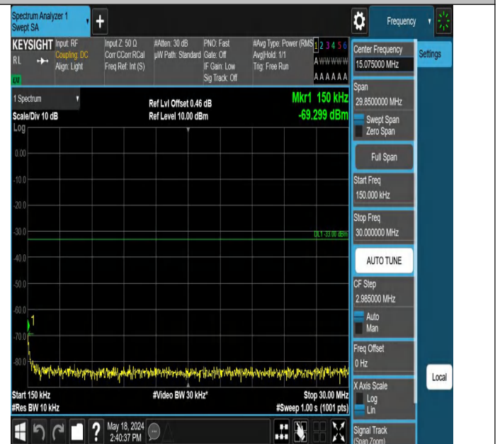
Band4_3MHz_QPSK_20385_1RB#0_0.15~30_0.15~30
