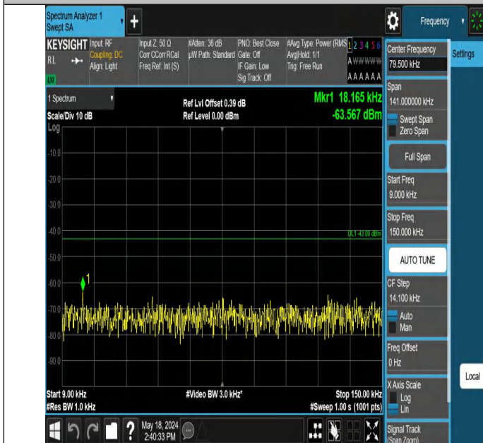
Band4_3MHz_QPSK_20385_1RB#0_0.009~0.15_0.009~0.15
