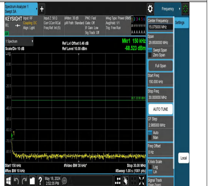
Band4_10MHz_QPSK_20000_1RB#0_0.15~30_0.15~30
