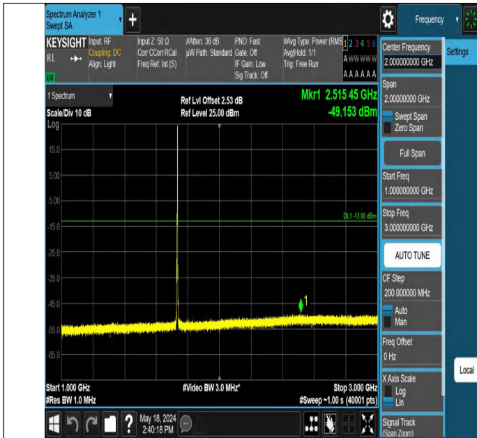
Band4_3MHz_QPSK_20175_1RB#14_1000~3000_1000~3000
