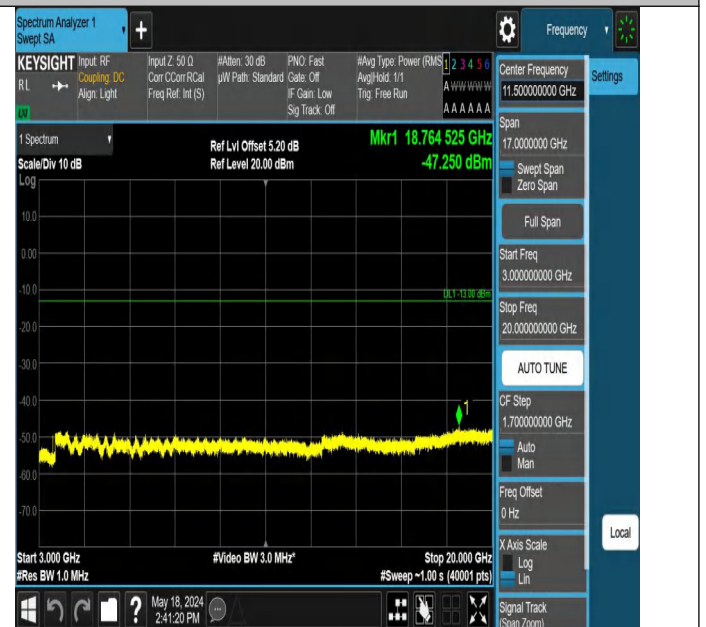
Band4_3MHz_QPSK_20385_1RB#14_3000~20000_3000~20000
