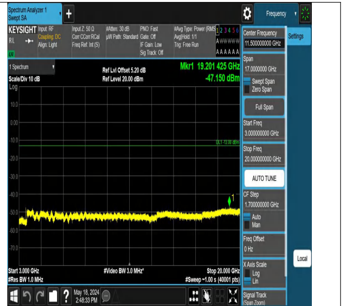
Band4_5MHz_QPSK_20375_1RB#24_3000~20000_3000~20000
