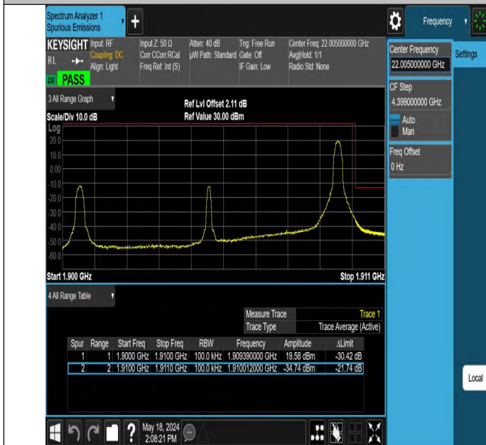
Band2_10MHz_QPSK_19150_1RB#49
