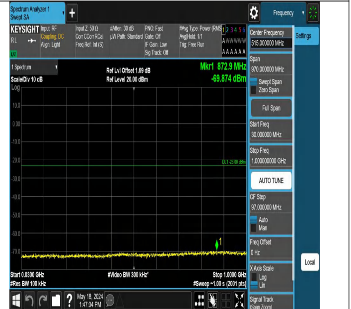
Band2_1.4MHz_QPSK_18607_1RB#5_30~1000_30~1000
