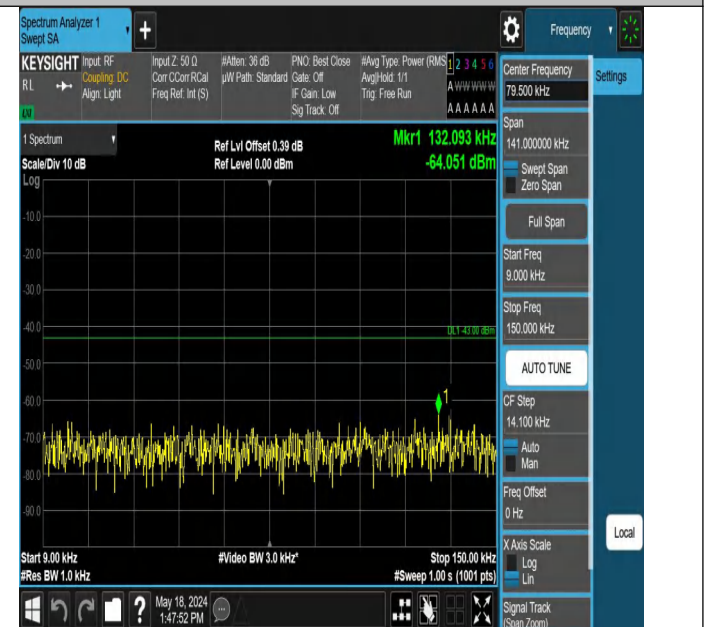
Band2_1.4MHz_QPSK_18900_1RB#5_0.009~0.15_0.009~0.15
