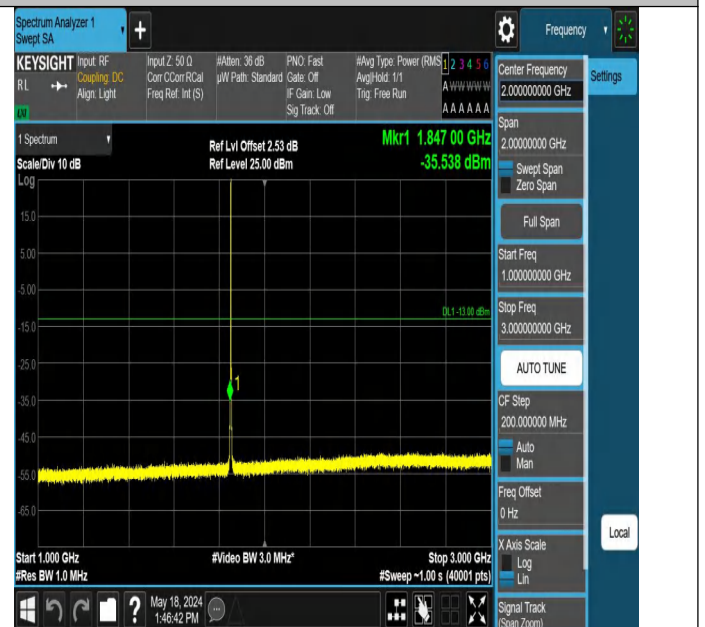
Band2_1.4MHz_QPSK_18607_1RB#0_1000~3000_1000~3000
