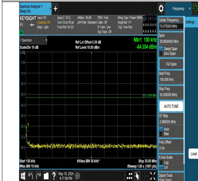
Band4-1513-3-0.15~30MHz-PASS
