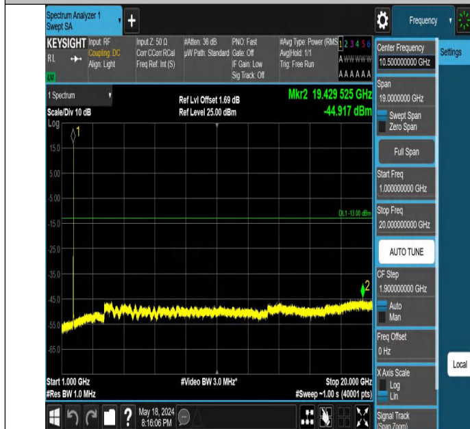
Band4-1312-3-1000~20000MHz-PASS
