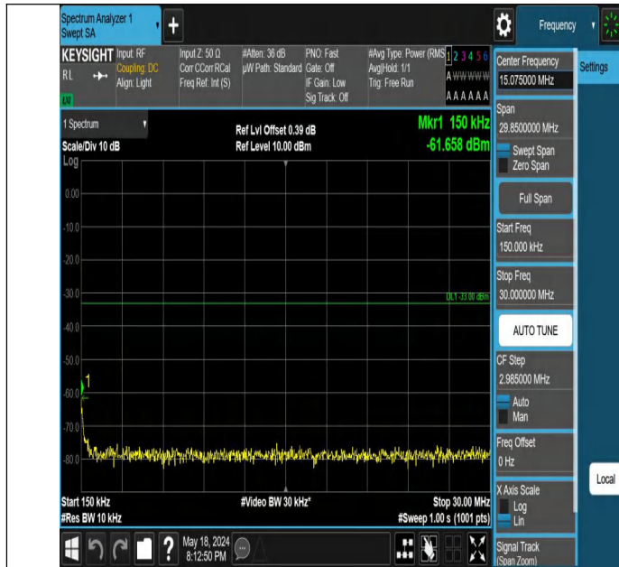
Band4-1513-1-0.15~30MHz-PASS
