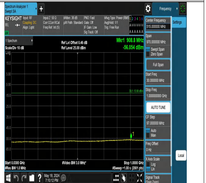
Band2-9400-2-30~1000MHz-PASS
