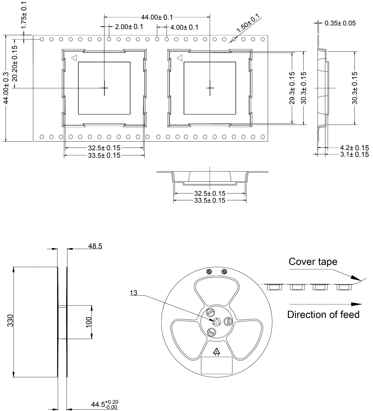
Figure 38: Carrier Tape
