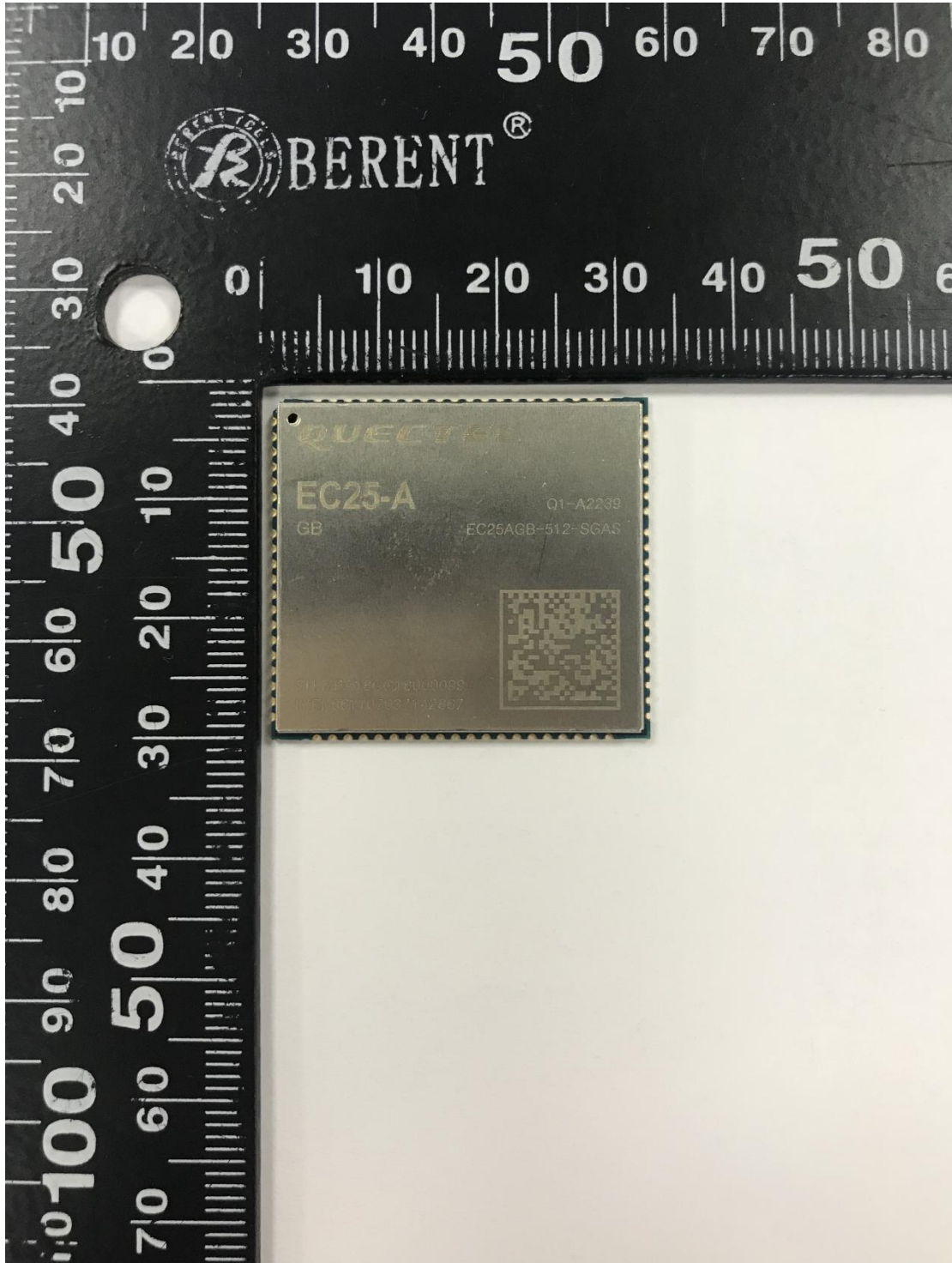
Front Side
