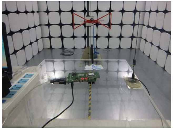
Radiated Spurious Emissions Test Setup Above 1GHz - 3
