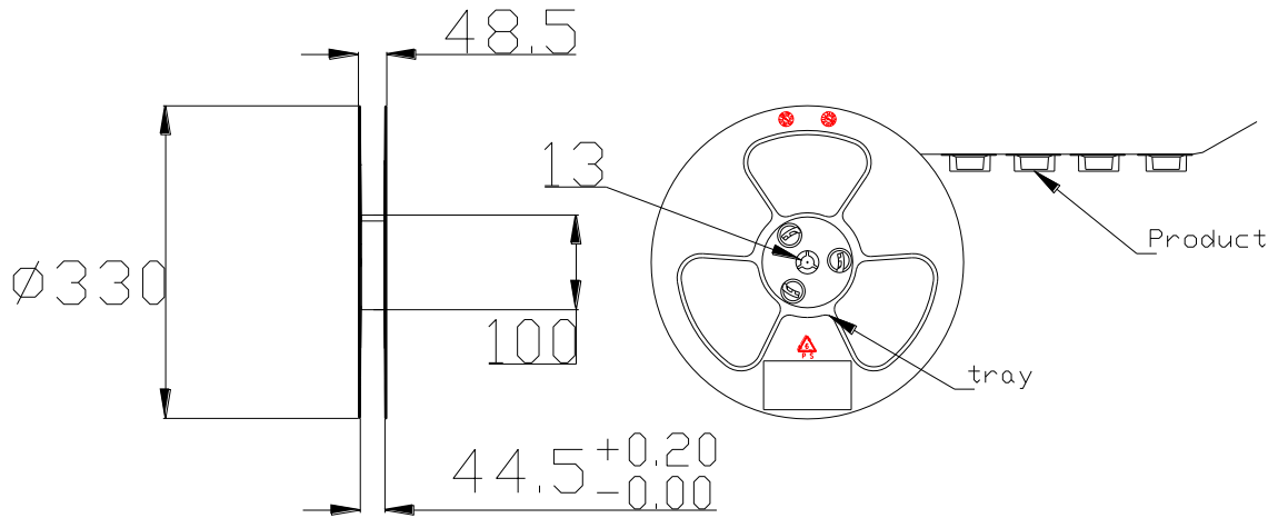
Figure 43: Dimensions of Reel
