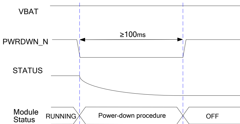
Figure 15: Timing of Emergency Shutdown
