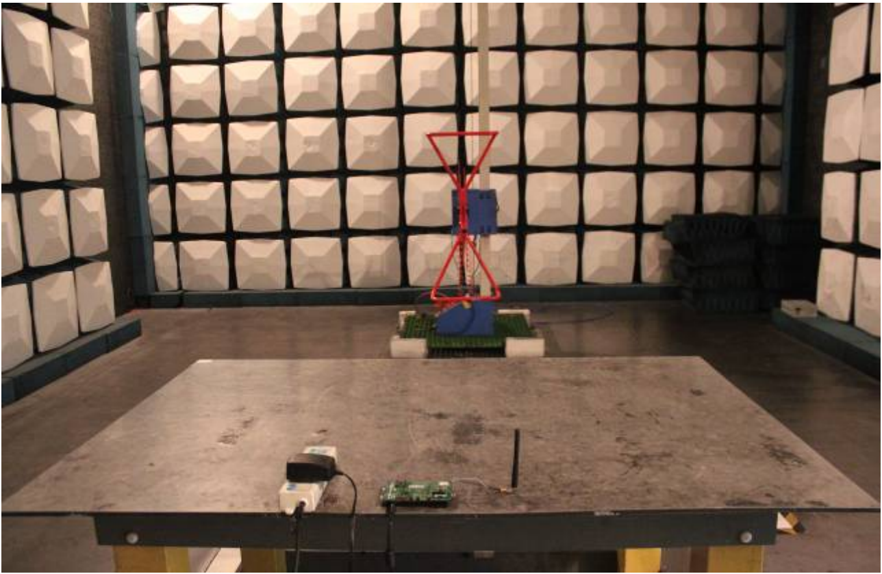
RADIATED EMISSION TEST
