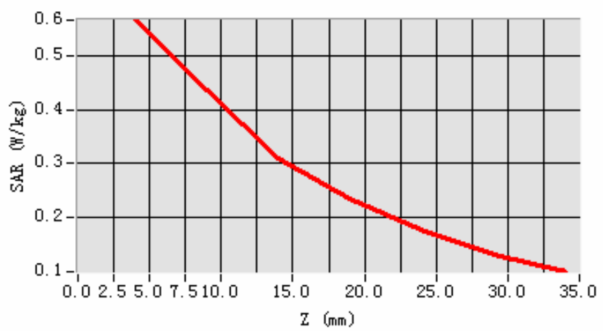
SAR, Z Axis Scan (X = -37, Y = -16)
