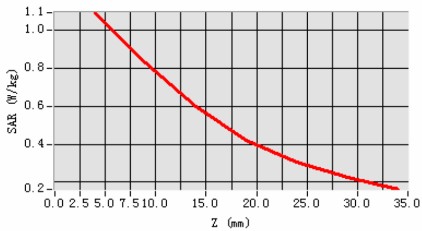
SAR, Z Axis Scan (X = -45, Y = -22)
