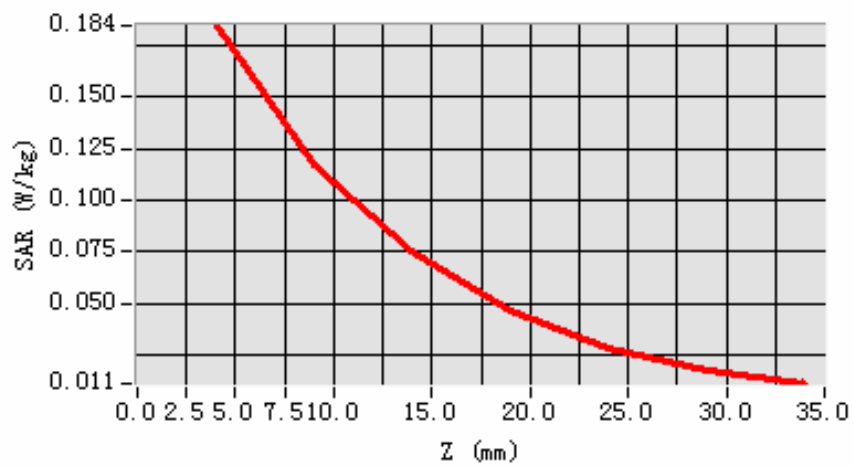
SAR, Z Axis Scan (X = -47, Y = -28)
