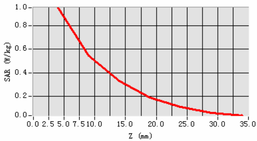
SAR, Z Axis Scan (X = -54, Y = -35)
