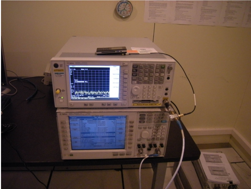
RF TEST
