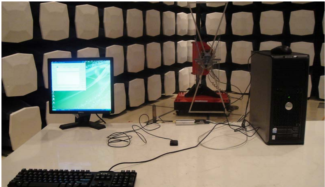
RADIATED EMISSION TEST
