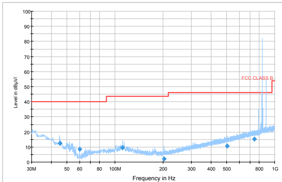
(Plot B: Test Antenna Horizontal)
