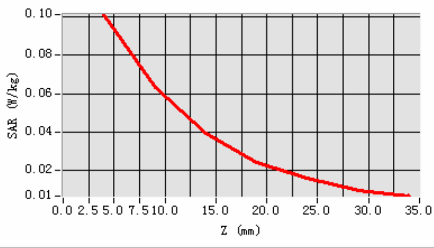
SAR, Z Axis Scan (X = 3, Y = 6)
