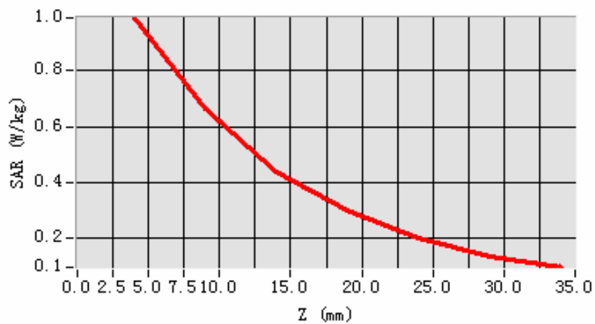
SAR, Z Axis Scan (X = -43, Y = -25)
