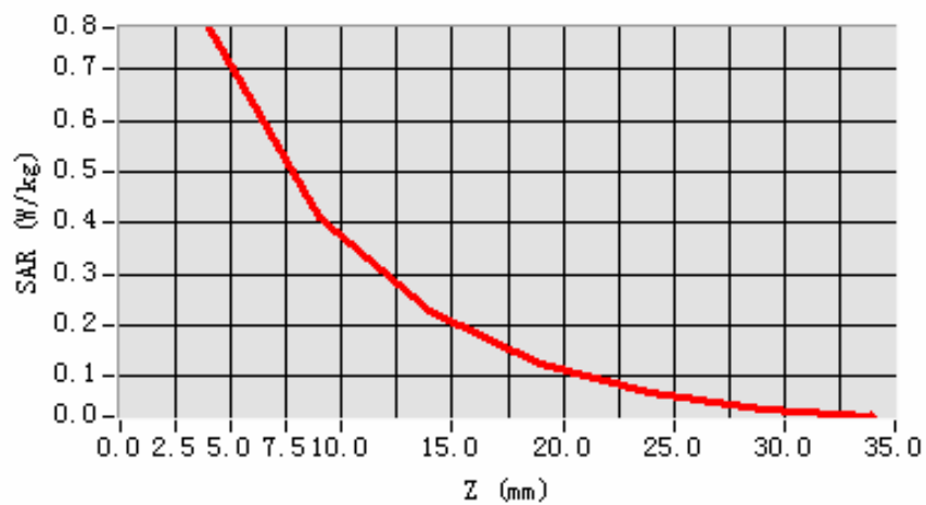
SAR, Z Axis Scan (X = -49, Y = -21)
