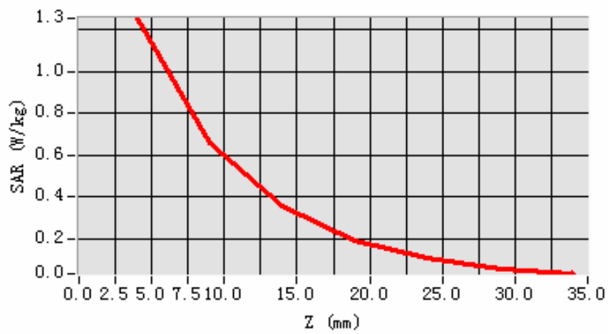
SAR, Z Axis Scan (X = -43, Y = -26)
