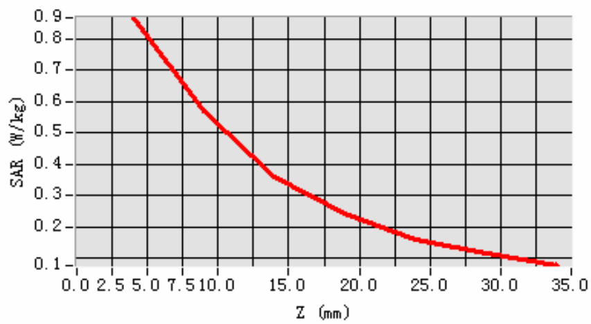
SAR, Z Axis Scan (X = -47, Y = -29)
