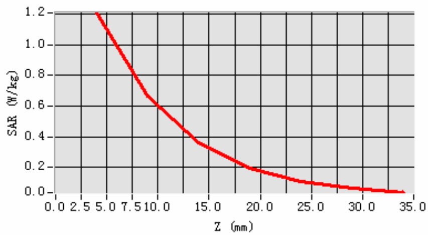
SAR, Z Axis Scan (X = -42, Y = -25)
