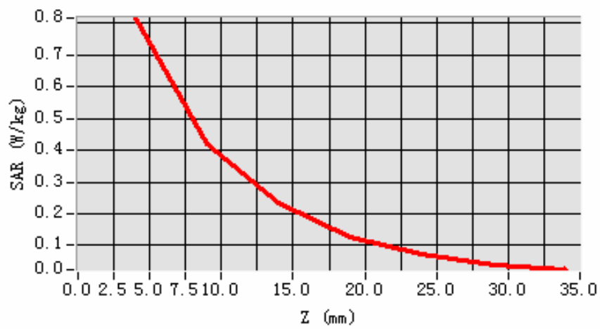
SAR, Z Axis Scan (X = -49, Y = -19)
