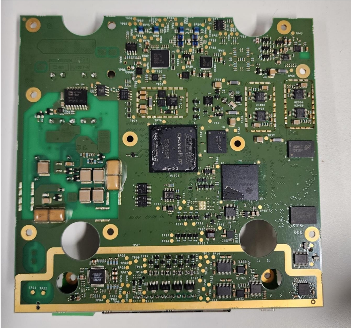
Digital Board back face
