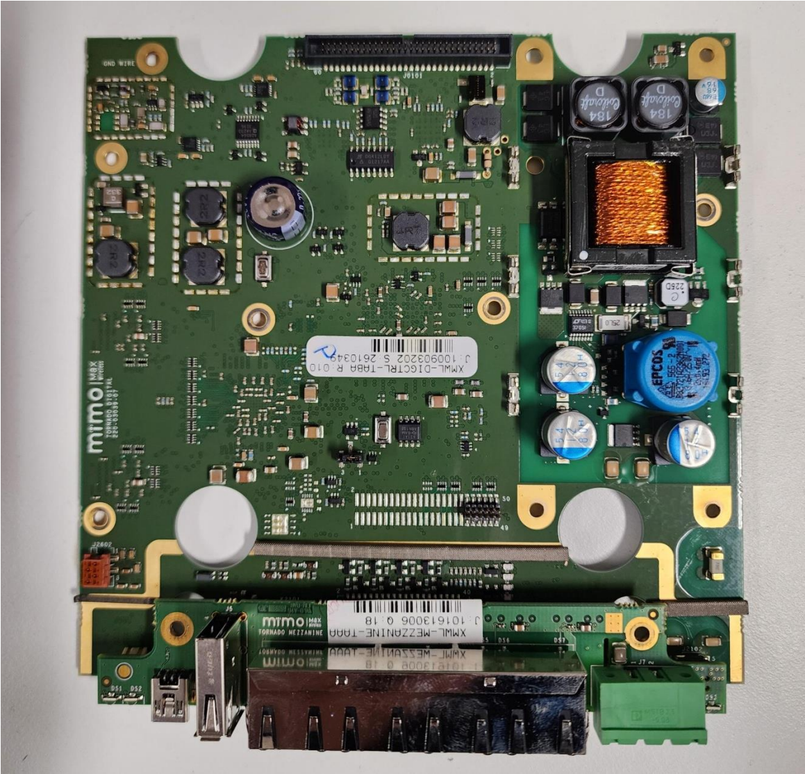
Digital Board top face
