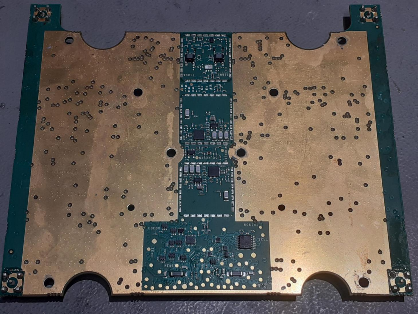
RF board back
