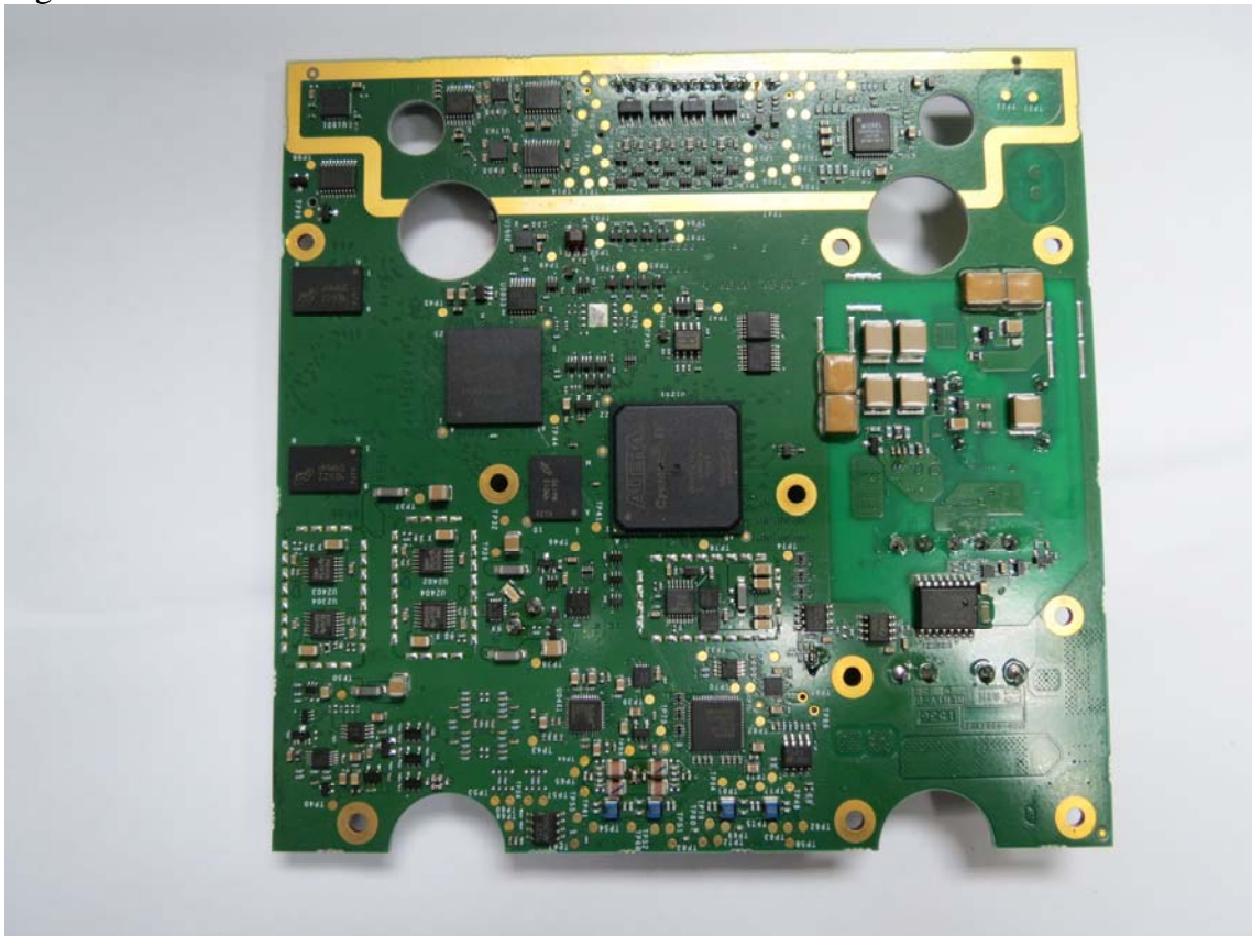
Digital board bottom side no shields
