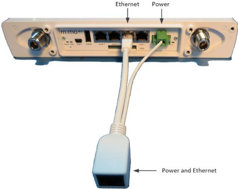
PoE Splitter
