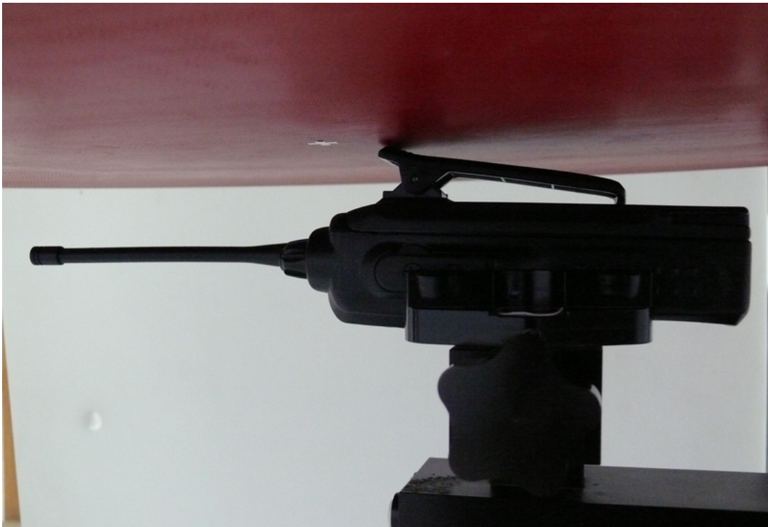
Picture 4: Face-held, The EUT display towards phantom, the distance from EUT to the bottom of the Phantom is 15mm
