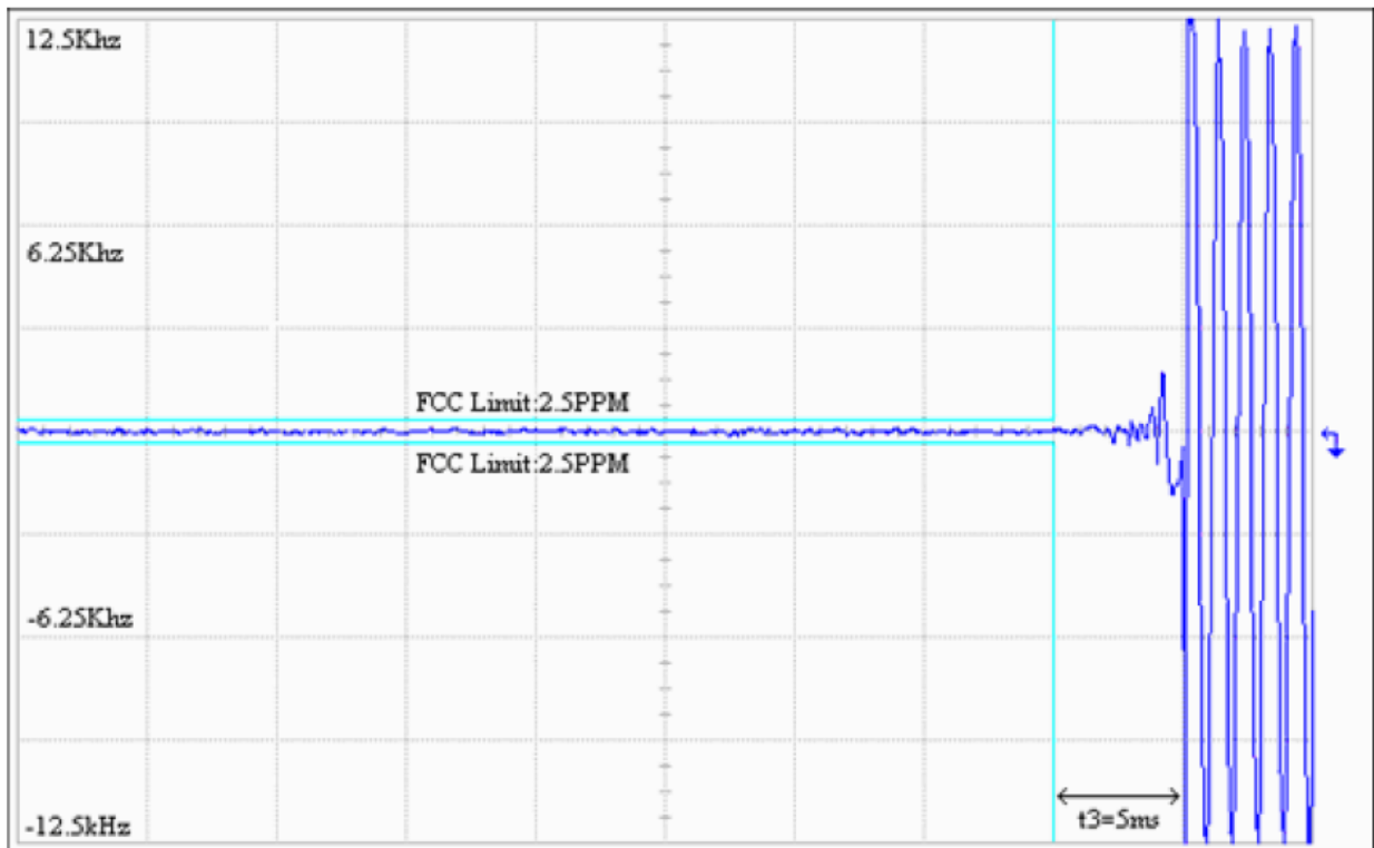
Transmitter Frequency Behaviour @ 12.5 KHz Channel Separation-----On - Off
