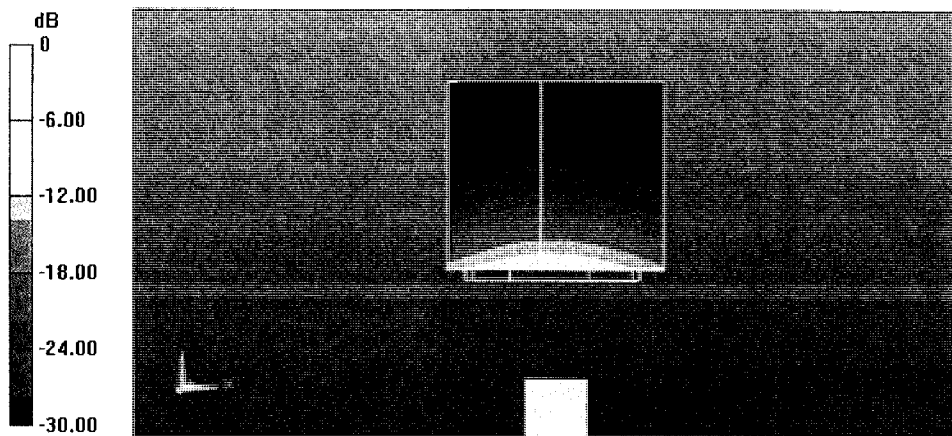
0 dB = 18.7 W/kg = 12.72 dBW/kg
