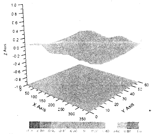
Uncertainty of Spherical Isotropy Assessment: \pm 2.8\% (K=2)
