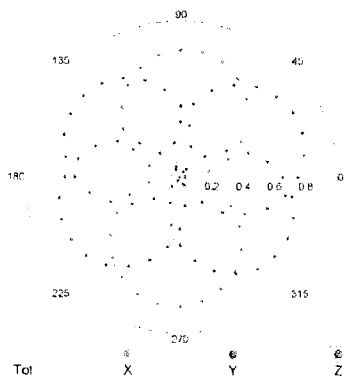
f=600 MHz,TEM
