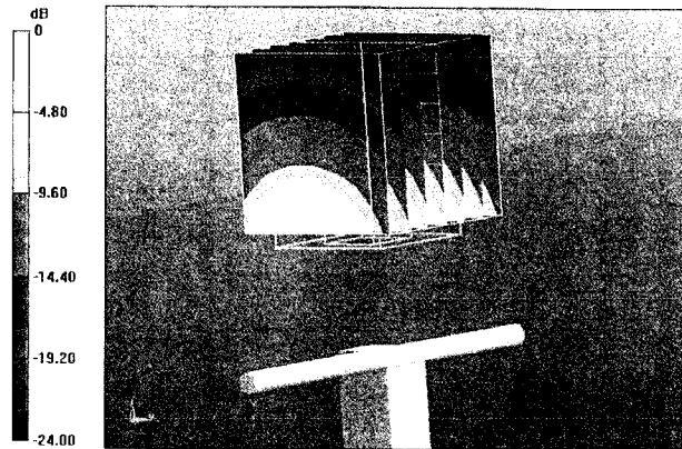
0 dB = 17.1 W/kg = 12.33 dBW/kg
