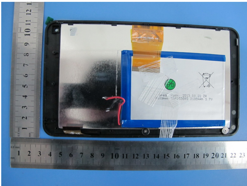
Photo 20 Appearance of Screen and Battery
