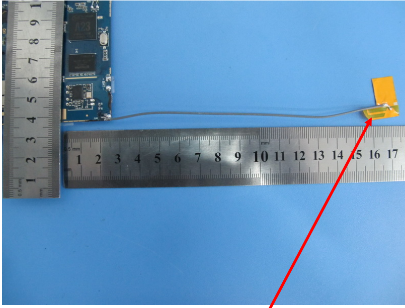
WiFi (2.4G) Antenna
