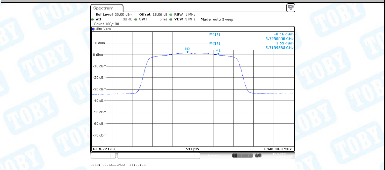
11N20SISO_Ant1_5720_UNII-3
