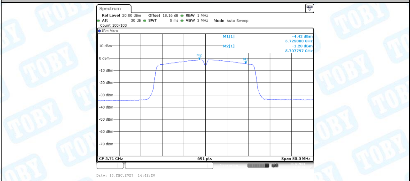
11N40SISO_Ant1_5710_UNII-3
