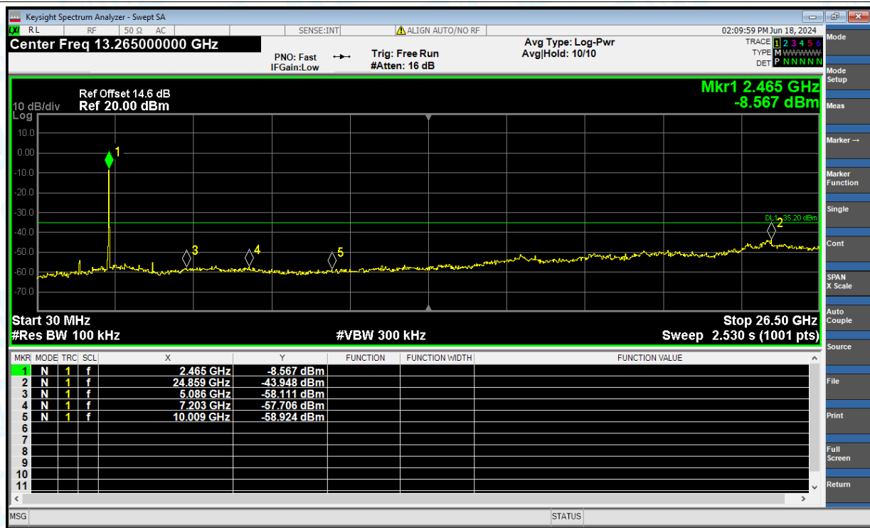
Tx. Spurious NVNT ax(VHT20) 2462MHz Ant1 Emission
