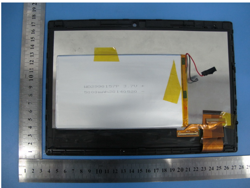
Photo 16 Appearance of Battery and Screen
