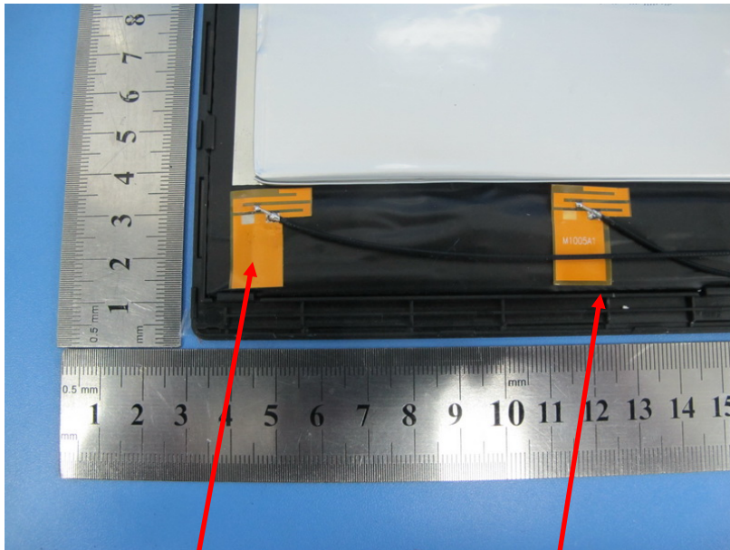
BT(2.4G) Antenna
