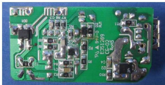
PCB side 2
