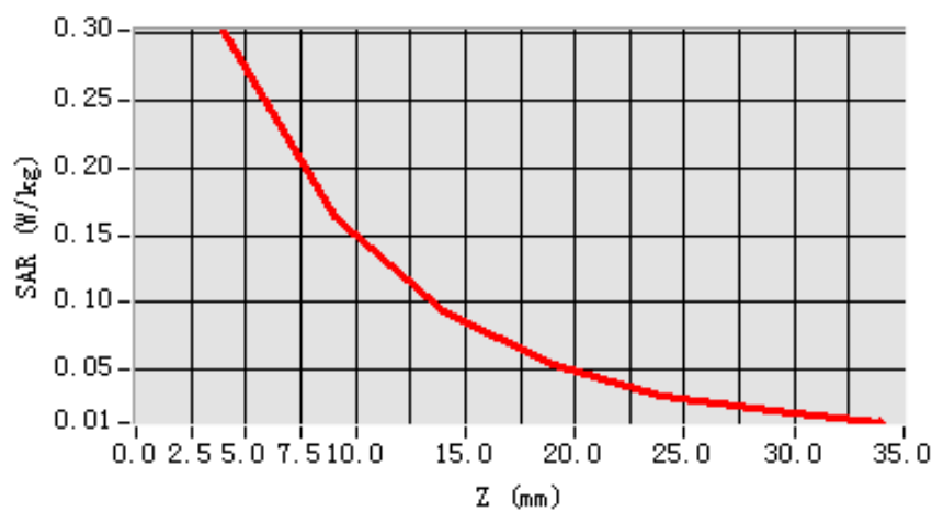
SAR, Z Axis Scan (X = -5, Y = -49)
