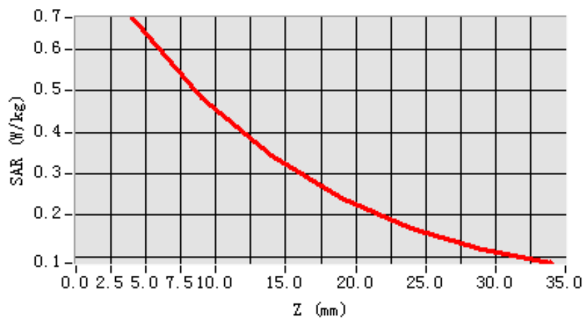
SAR, Z Axis Scan (X = -20, Y = -1)
