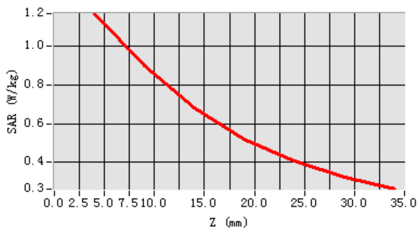
SAR, Z Axis Scan (X = -20, Y = -16)
