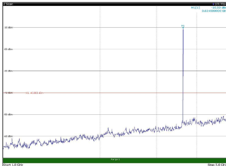
Channel: MIDDLE, Modulation: QPSK, BW=15MHz, Range: 1GHz - 5GHz, Polarization: Vertical
