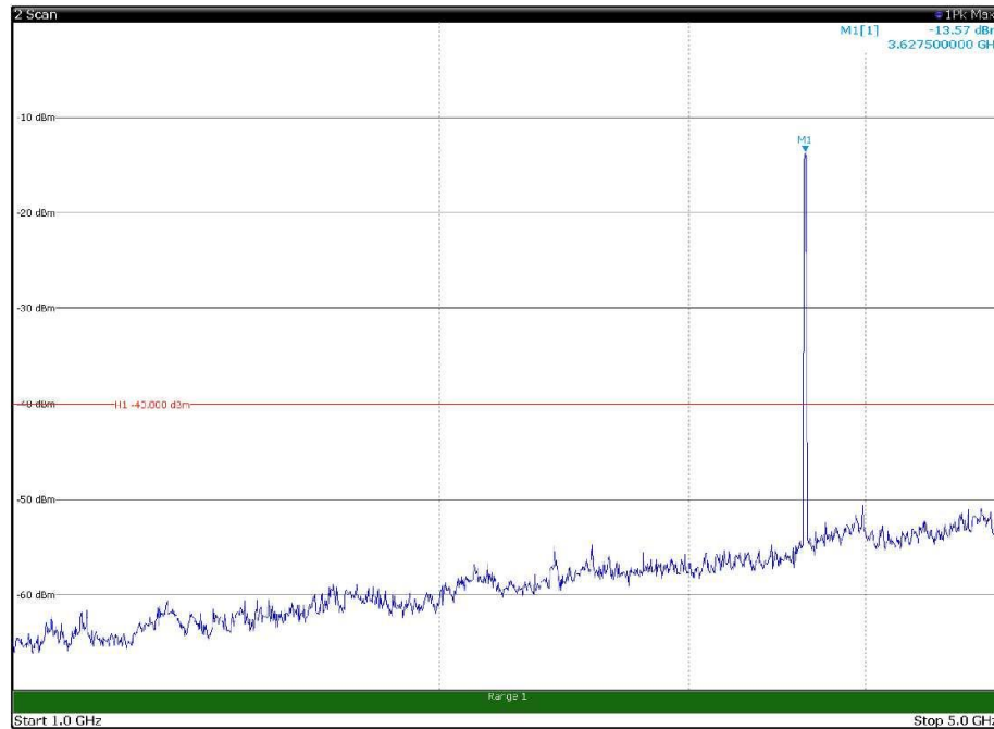
Channel: MIDDLE, Modulation: QPSK, BW=15MHz, Range: 1GHz - 5GHz, Polarization: Horizontal
