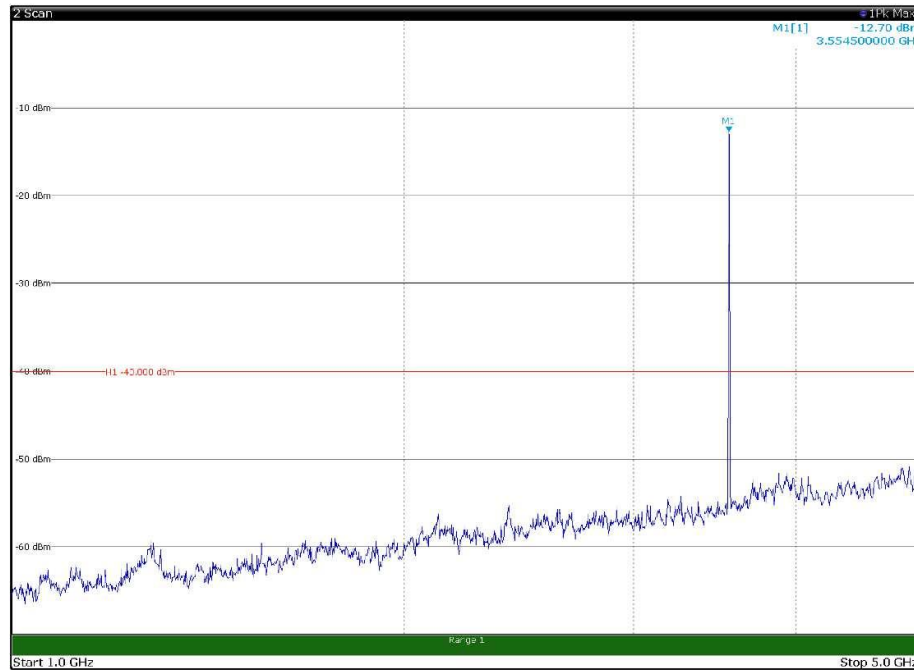
Channel: BOTTOM, Modulation: 256QAM, BW=10MHz, Range: 1GHz - 5GHz, Polarization: Horizontal
