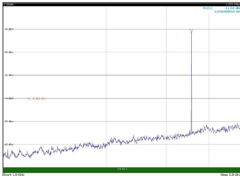
Channel: BOTTOM, Modulation: 256QAM, BW=10MHz, Range: 1GHz - 5GHz, Polarization: Vertical
