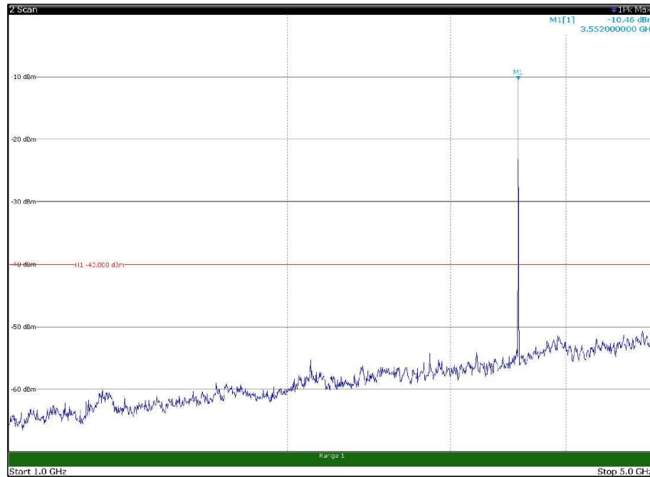
Channel: BOTTOM, Modulation: 16QAM, BW=5MHz, Range: 1GHz - 5GHz, Polarization: Horizontal
