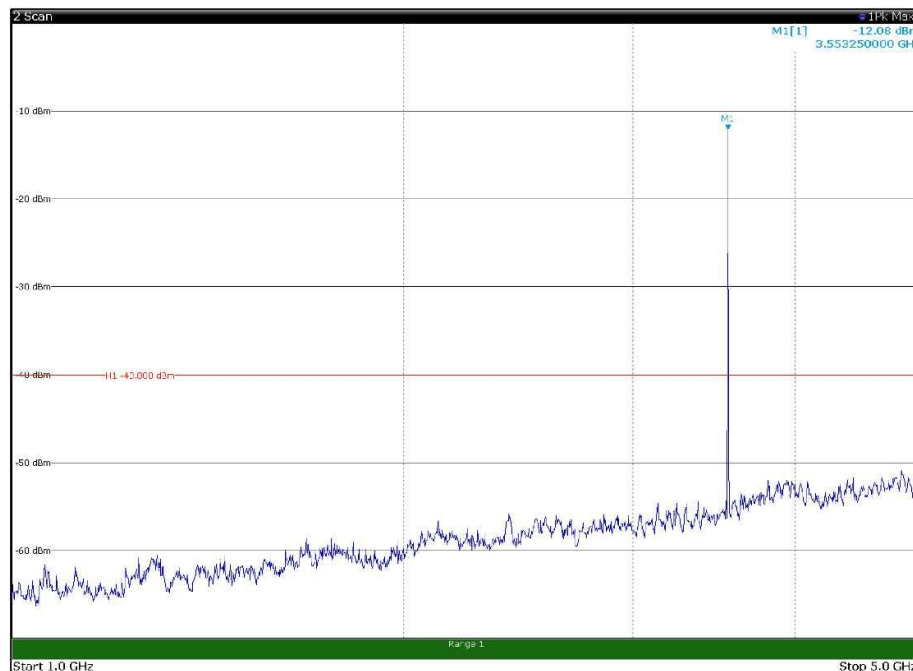
Channel: BOTTOM, Modulation: 16QAM, BW=5MHz, Range: 1GHz - 5GHz, Polarization: Vertical
