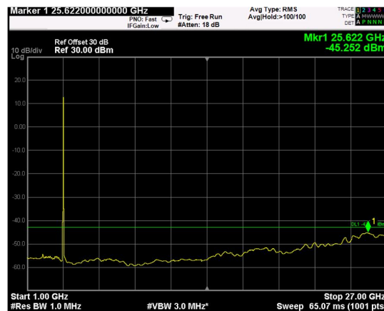
Channel: BOTTOM, Modulation: 256QAM, BW=15MHz, Range: 1GHz - 27GHz
