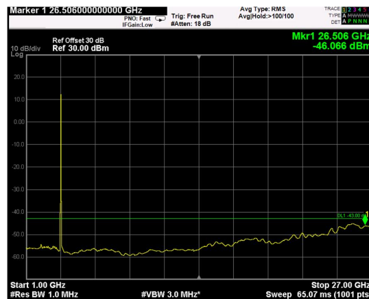
Channel: MIDDLE, Modulation: 64QAM, BW=10MHz, Range: 1GHz - 27GHz
