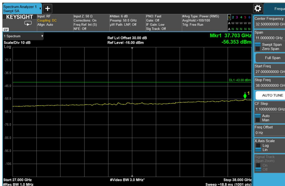
Channel: BOTTOM, Modulation: QPSK, BW=15MHz, Range: 27GHz - 38GHz
