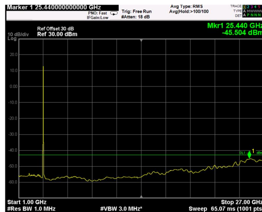
Channel: TOP, Modulation: 256QAM, BW=10MHz, Range: 1GHz - 27GHz
