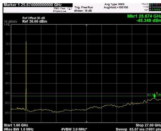
Channel: BOTTOM, Modulation: QPSK, BW=20MHz, Range: 1GHz - 27GHz
