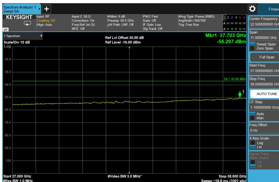
Channel: BOTTOM, Modulation: 64QAM, BW=15MHz, Range: 27GHz - 38GHz
