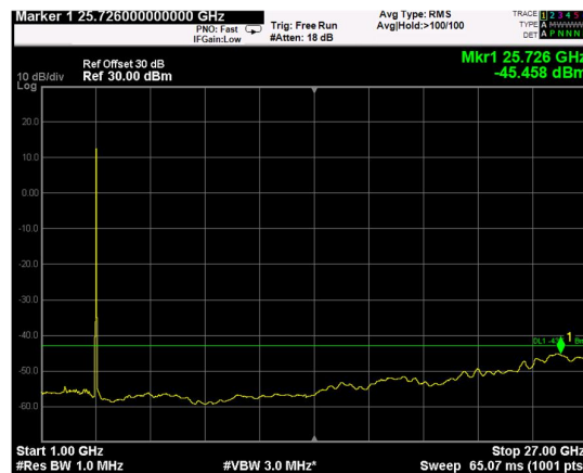
Channel: TOP, Modulation: QPSK, BW=15MHz, Range: 1GHz - 27GHz
