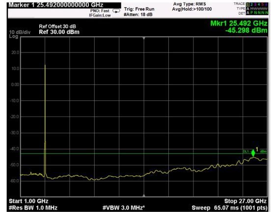
Channel: BOTTOM, Modulation: 16QAM, BW=15MHz, Range: 1GHz - 27GHz
