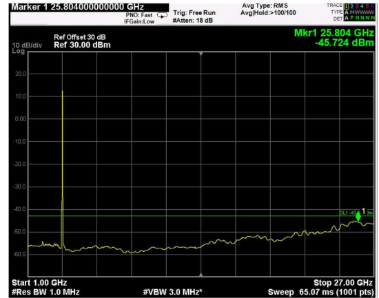
Channel: TOP, Modulation: 16QAM, BW=20MHz, Range: 1GHz - 27GHz
