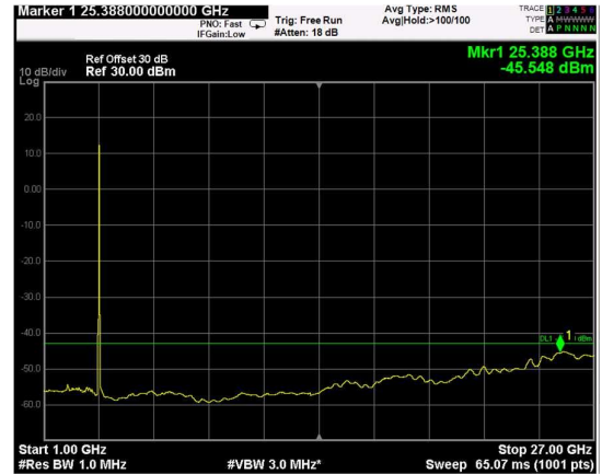
Channel: TOP, Modulation: QPSK, BW=15MHz, Range: 1GHz - 27GHz
