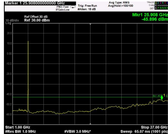
Channel: BOTTOM, Modulation: 64QAM, BW=15MHz, Range: 1GHz - 27GHz
