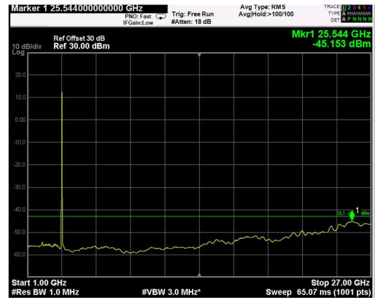
Channel: BOTTOM, Modulation: QPSK, BW=15MHz, Range: 1GHz - 27GHz
