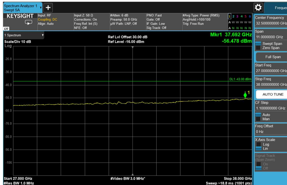
Channel: TOP, Modulation: 16QAM, BW=20MHz, Range: 27GHz - 38GHz
