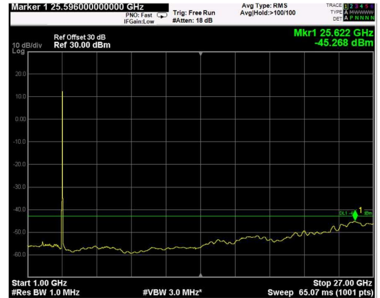
Channel: BOTTOM, Modulation: 64QAM, BW=20MHz, Range: 1GHz - 27GHz
